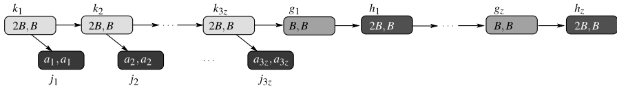
Fig. 6 The instance of malleable scheduling constructed from an instance of 3-PARTITION; the precedence constraints clearly form a caterpillar. All tasks j_i and g_i are oblivious of their allotment, while the processing time of all k_i and h_i is halved when using two processors
