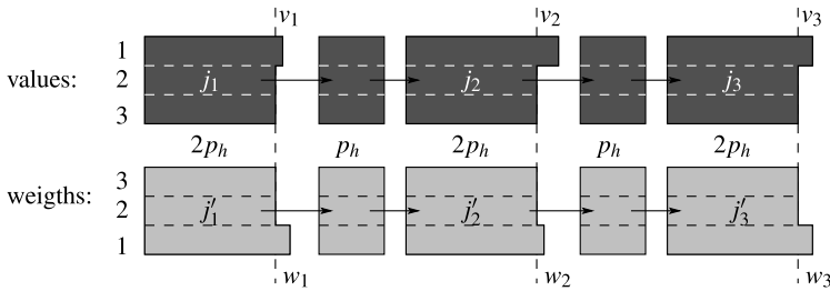
Fig. 4 The two chains of malleable tasks constructed from a KNAPSACK instance with processing times on one, two, and three processors. Every other element in each chain is oblivious of the allotment, while for the remaining tasks, allotting only one processor increases their processing time according to their knapsack value in one chain, and according to their knapsack weight in the other
